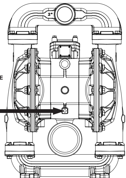
THE POSITION OF THE GROUND WIRE
